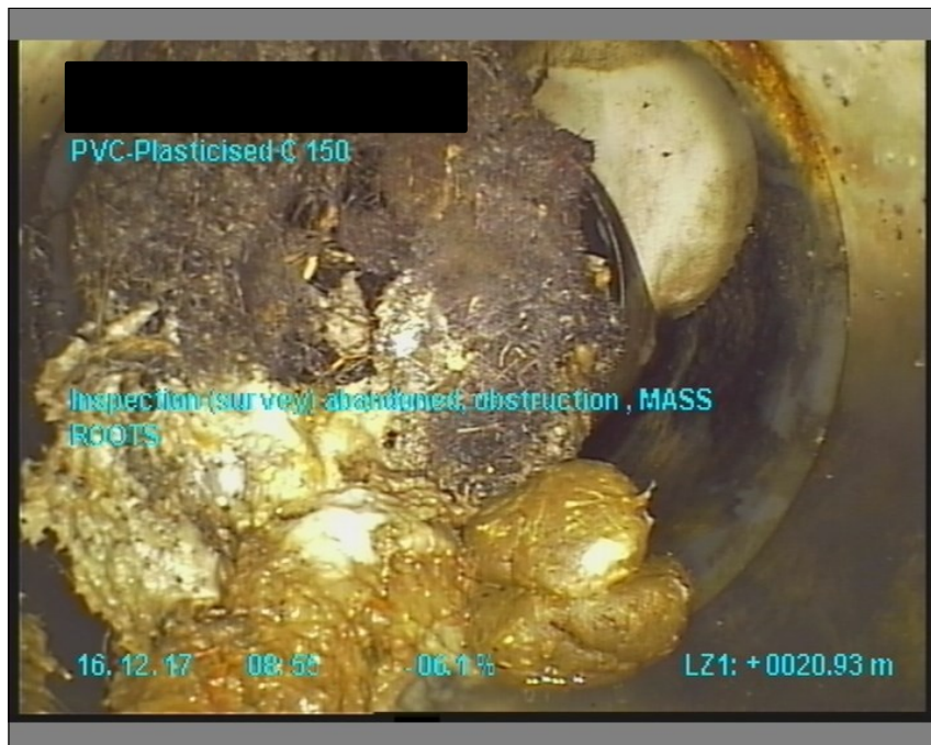
Photo: 085540_16122017_20.JPG 20.9m, Inspection (survey) abandoned, obstruction , MASS ROOTS
